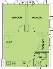
2 BR CORNER UNIT STANDARD 2 48 SQM
