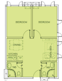
2 BR CORNER UNIT STANDARD 1 48 SQM
